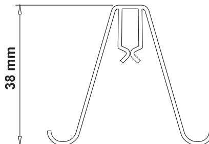
Tile supporter for T-Grid CODE: TA 68
